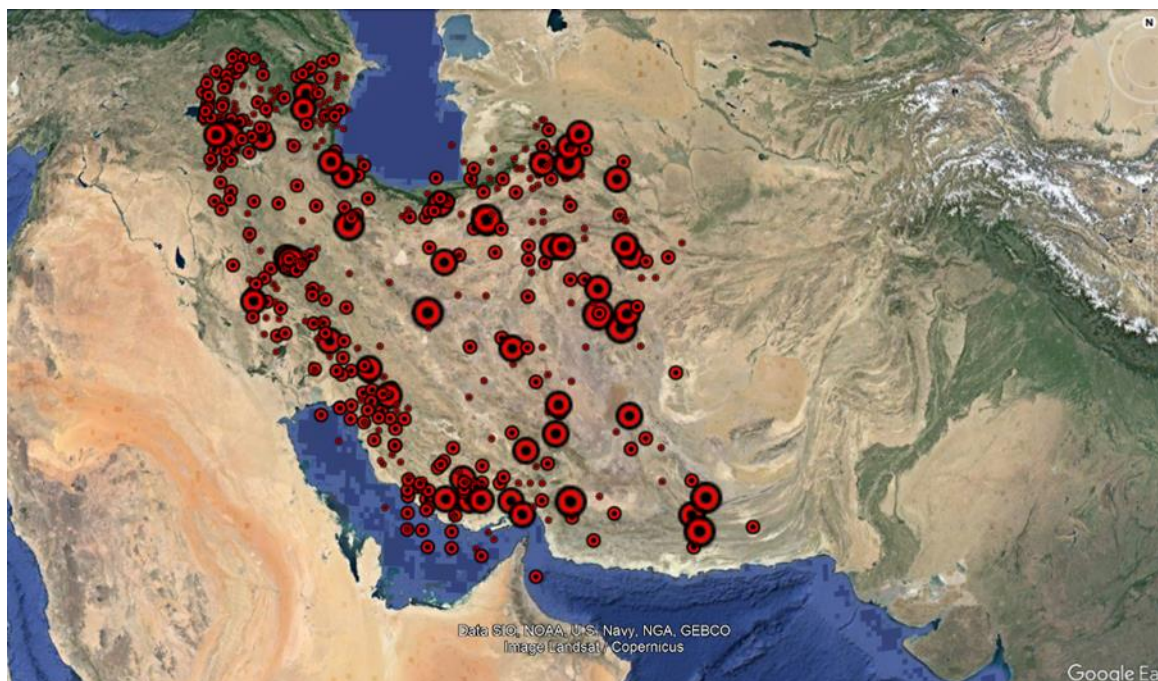
Figure 1: Recorded earthquakes 1900-1963
